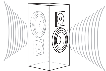
Fig 3 Bipole operation (no null)
