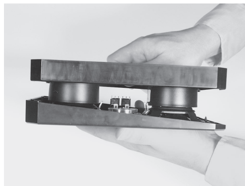
Fig 5 The mid/high baffle shown removed for clarity with the removable leveling spacer. The spacer can be removed for tilting without disconnecting the assembly from the speaker.
